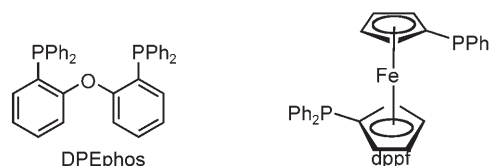
Figure 3. Structures of bidentate ligands DPEphos and dppf.
