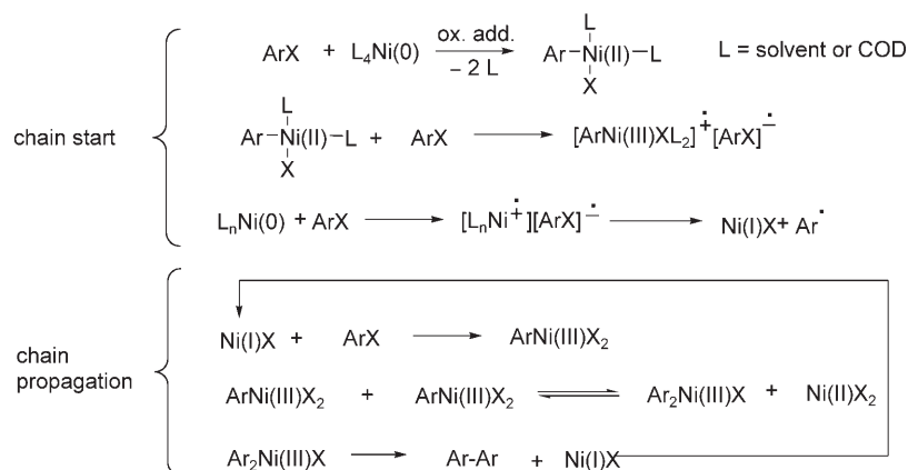
Scheme 1. Proposed mechanism of Ni(0)-mediated homocouplings of aryl halides using Ni(0) species. [26]
