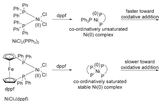
Figure 4. Difference in catalytic activity of coordinatively unsaturated and saturated Ni(0) complexes.
