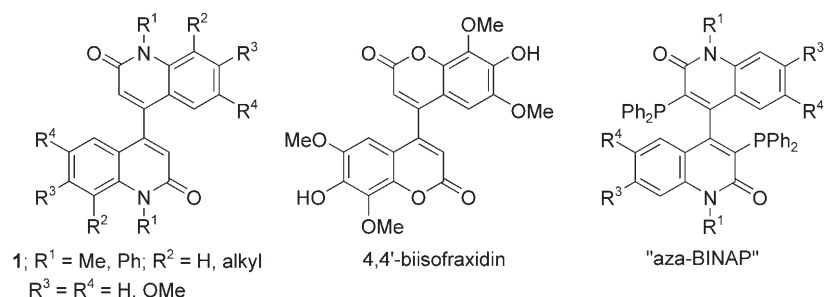
Figure 2. 4,4'-Bisquinolones and 4,4'-biscoumarins.
