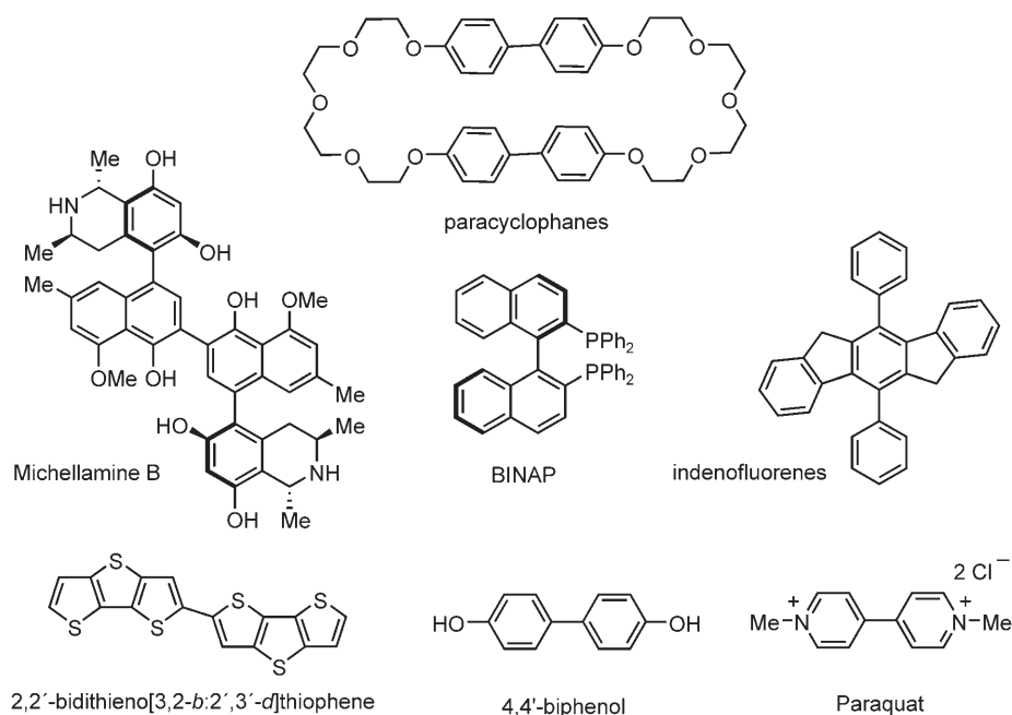
Figure 1. Important symmetrical biaryl products.
